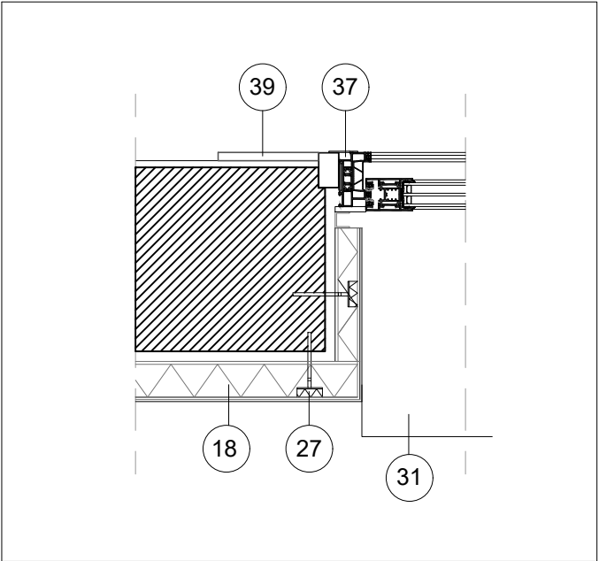
DETALL E (PLANTA BRANCAL)
