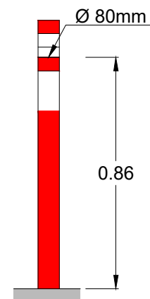
PILONA E:1/20
