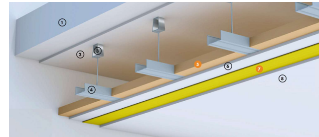
DETALL X - cel ras base
