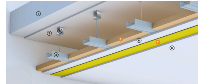
DETALL X - cel ras base
