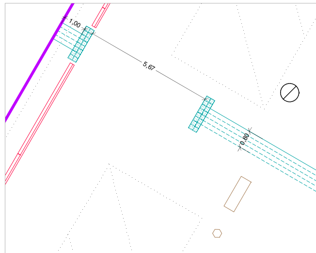
DETALL 3_ E:1/100
