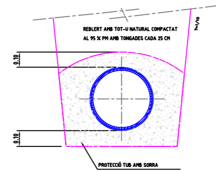
RASA CONDUCTE AIGUA POTABLE
