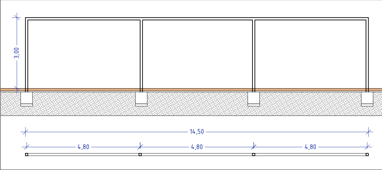
PORTIC 1 - 1:100
