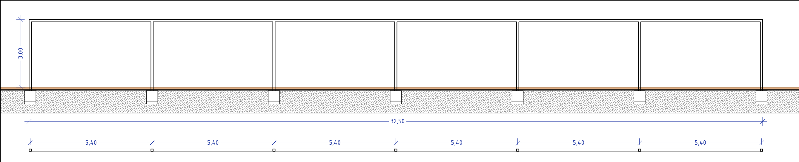
PORTIC 2 - 1:100
