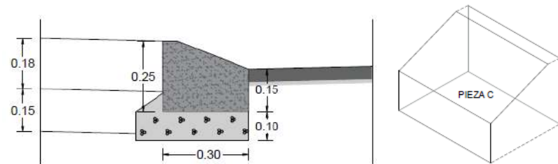
Figura 35. Detall vorada remuntable gual vehicles
