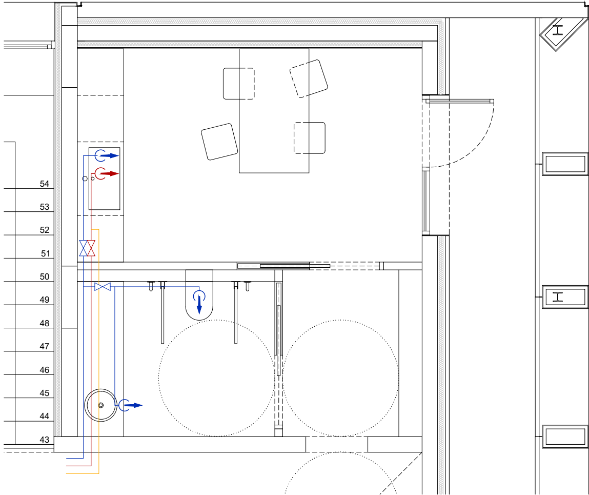
PLANTA AFS I ACS. OFFICE I BANY P1
