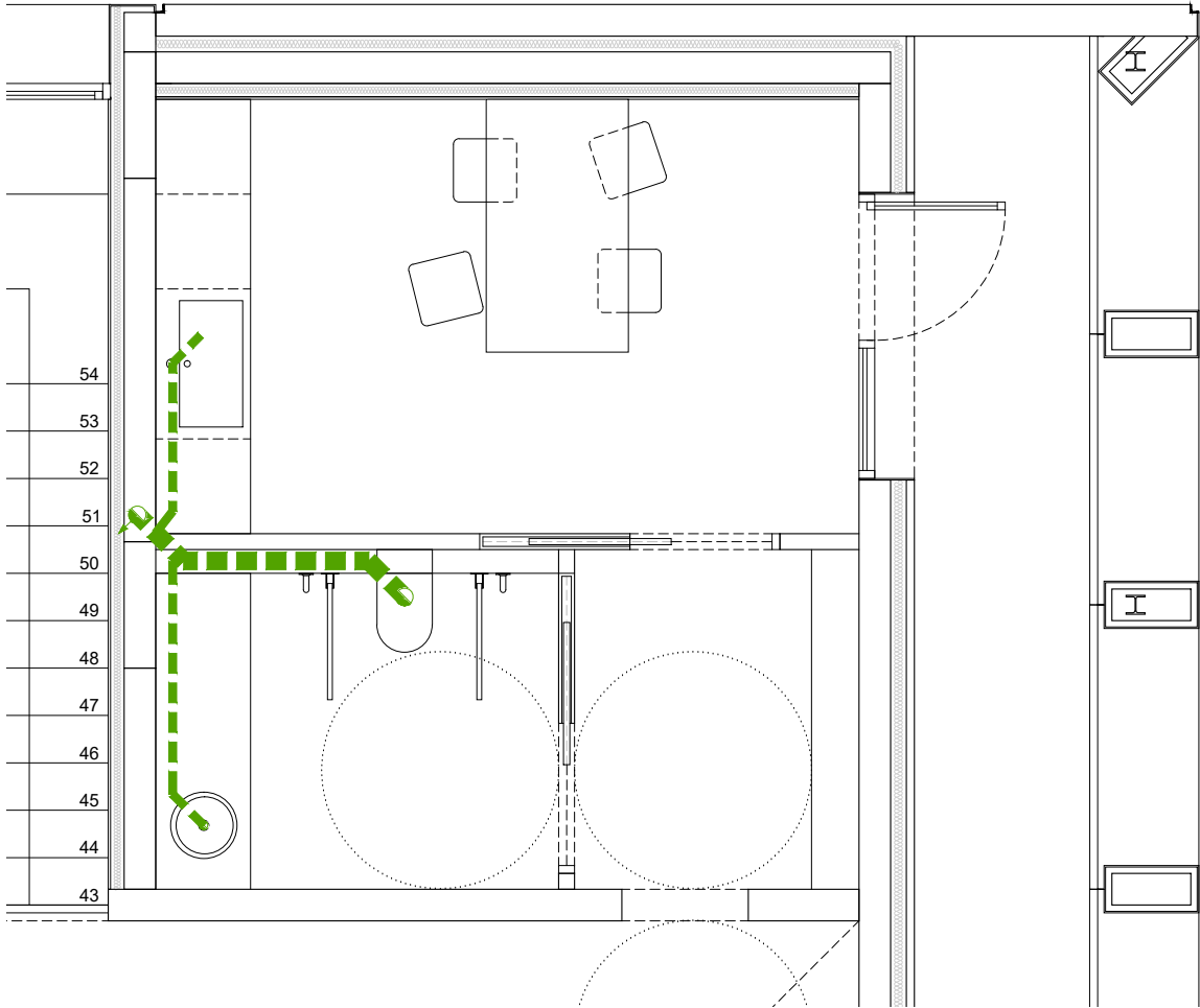
PLANTA SANEJAMENT. OFFICE I BANY P1
