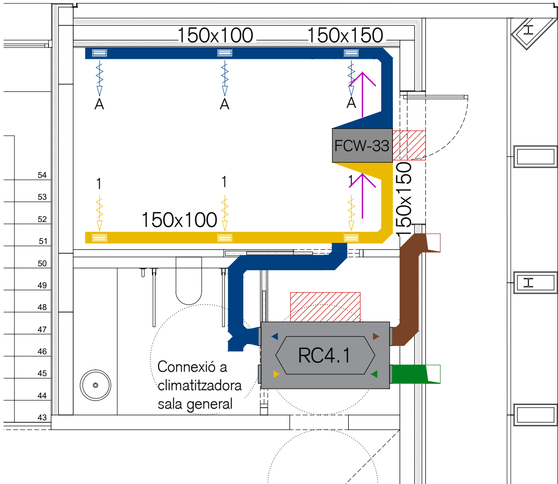
PLANTA CLIMA. OFFICE I BANY P1
