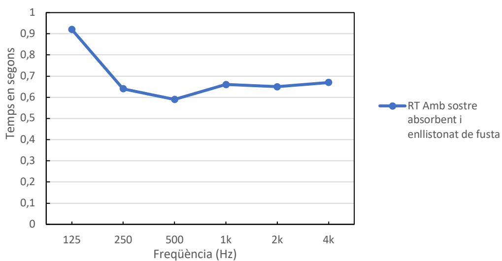
RT Sala Polivalent
