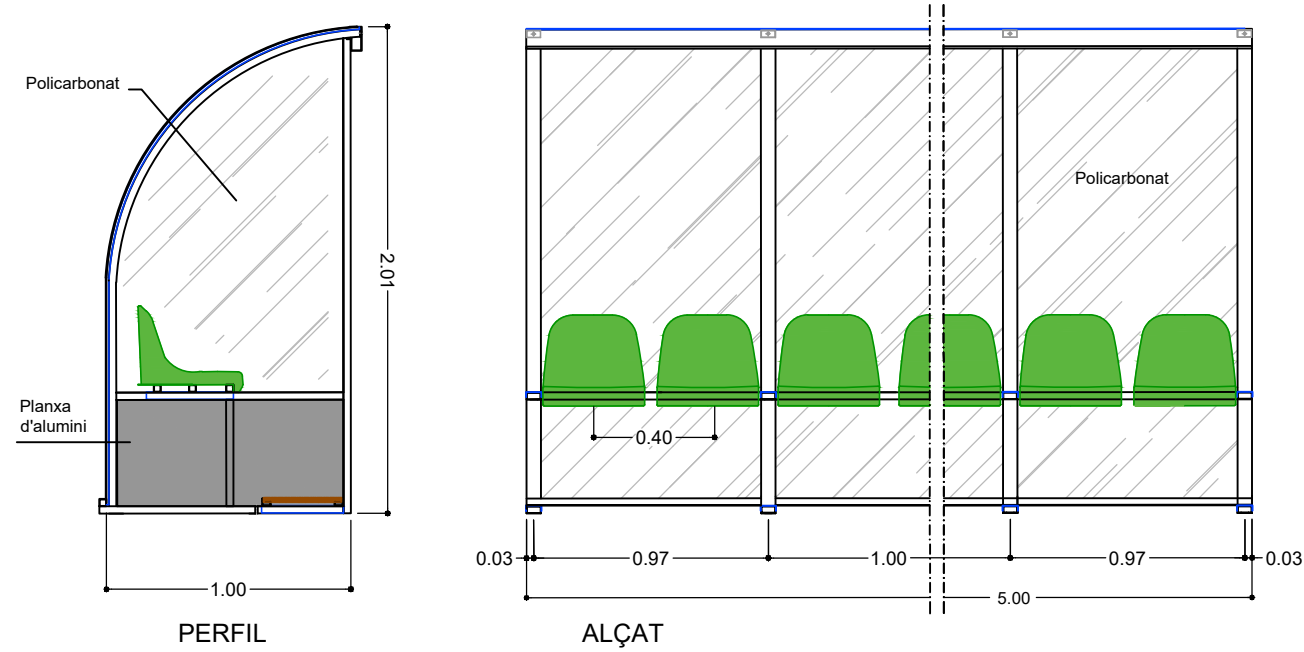
DETALL BANQUETES ( 10 PLACES )
