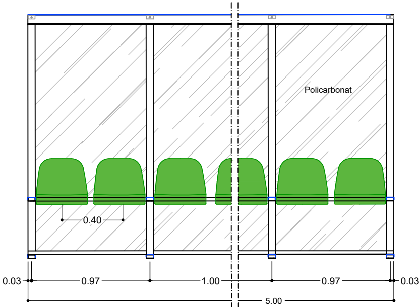
DETALL BANQUETES ( 10 PLACES )
