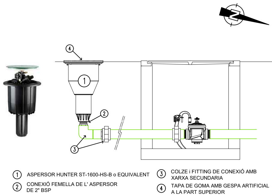
DETALL ASPERSOR EMERGENT (HUNTER ST-1600 o similar)
