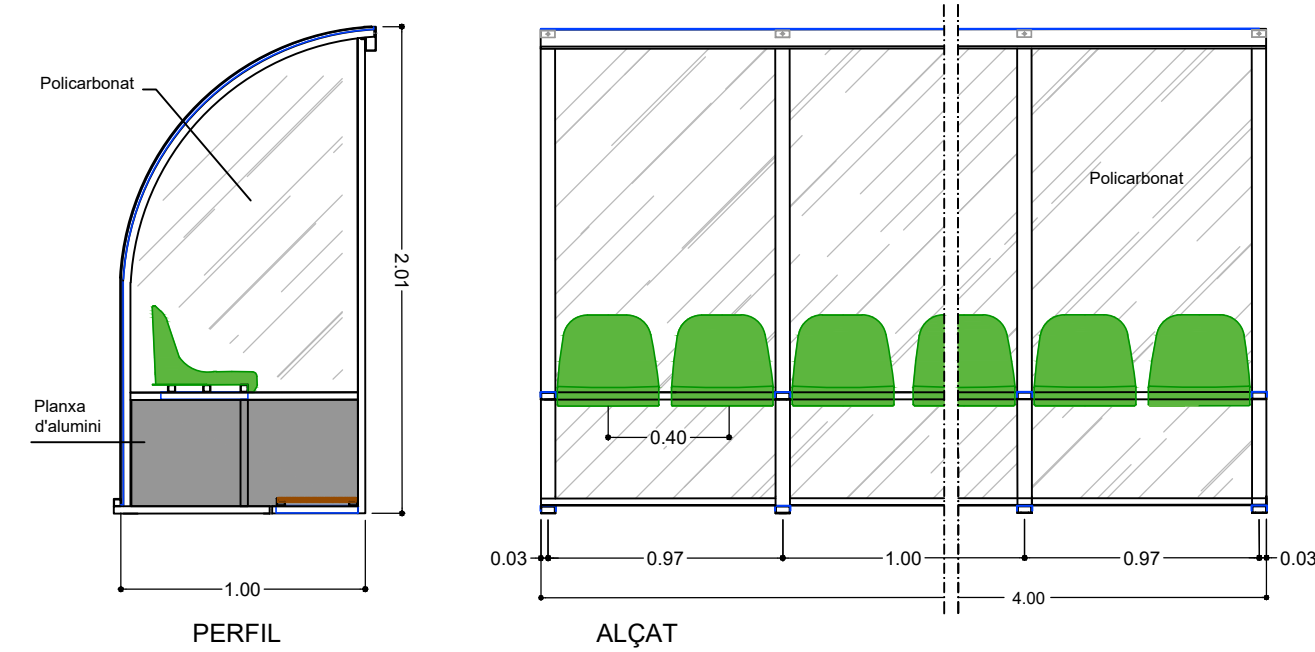
DETALL BANQUETES ( 8 PLACES )
