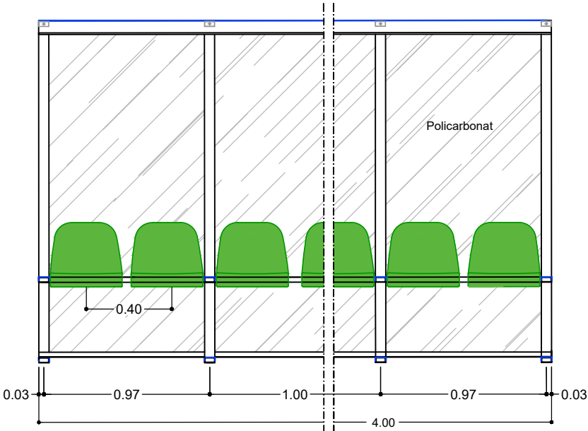
DETALL BANQUETES ( 8 PLACES )
