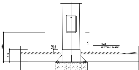
Columna i plaques base
