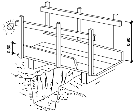
PASARELA PEATONAL
