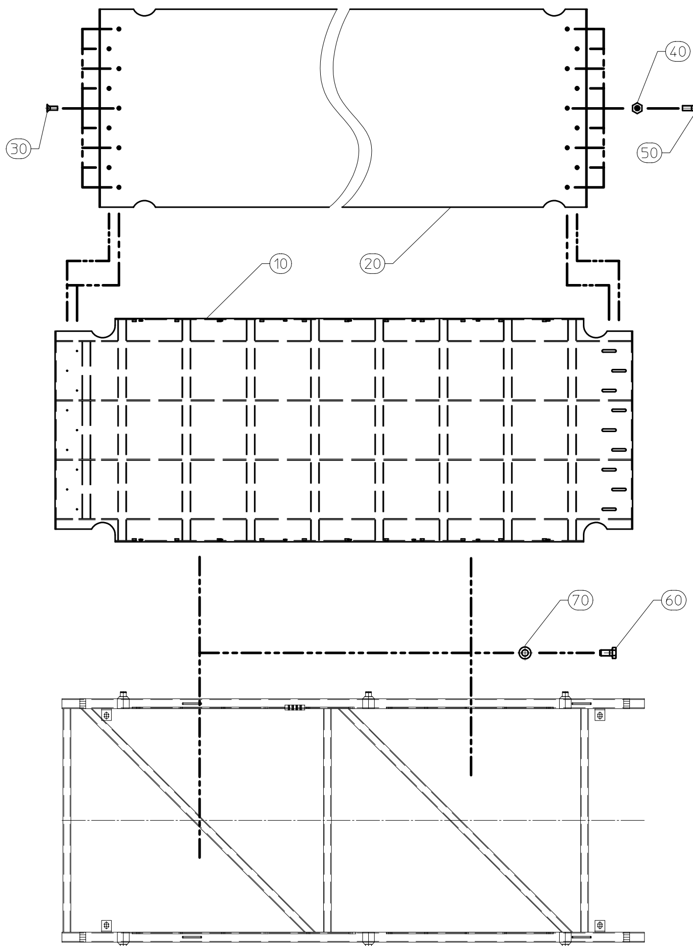
Austragsbandrahmen extraction belt frame
