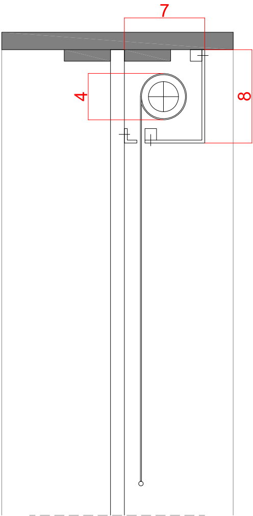
Detalle enrollables e 1/5
