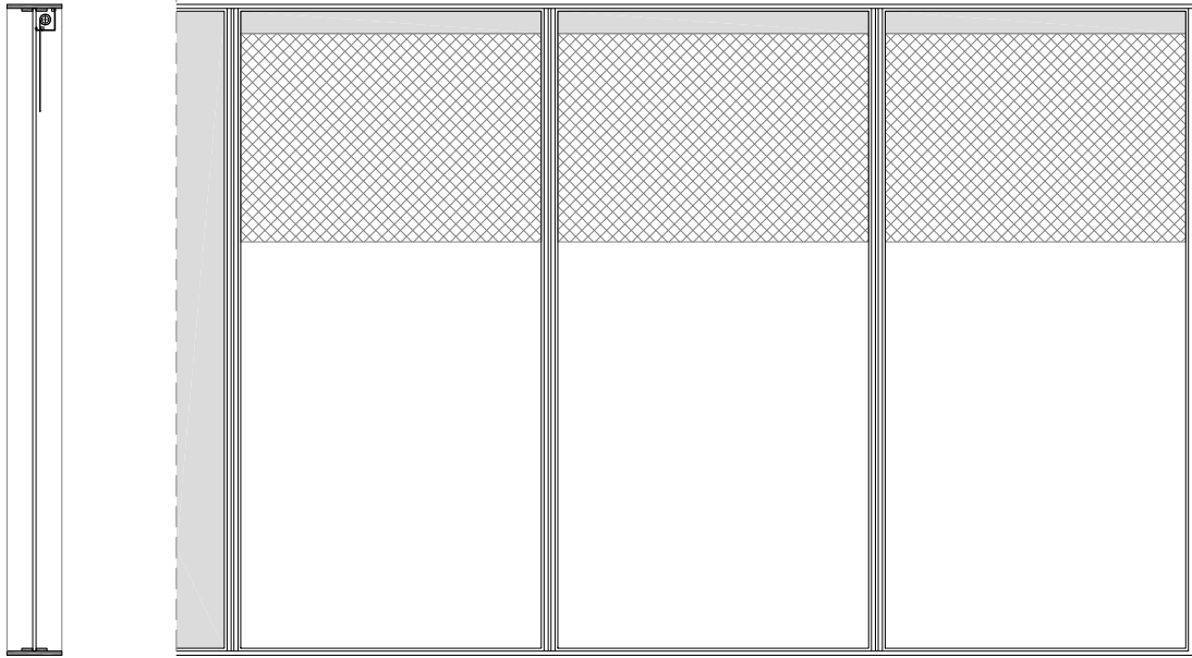
Detalle enrollables e 1/30
