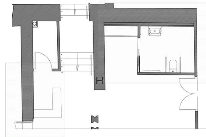
PLANTA: BARRA - ARMARI - BANY ACCESSIBLE
