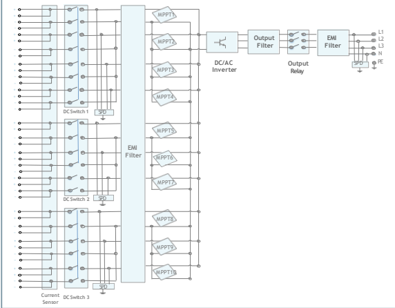
Circuit Diagram
