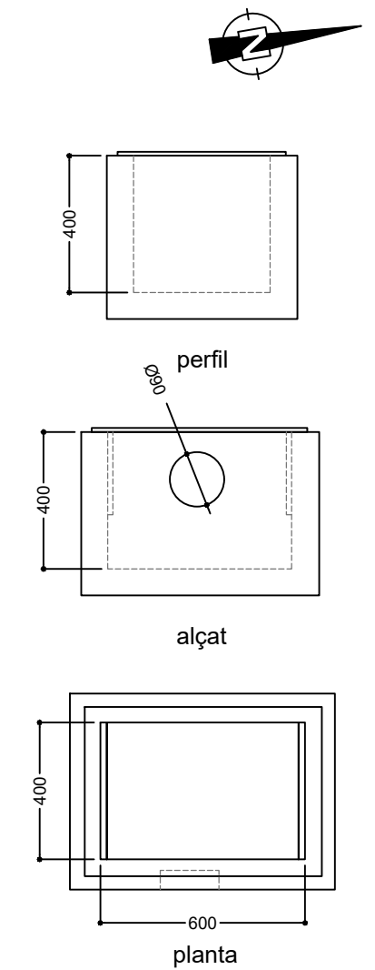
Detall Embornal 60x40x40h (int) e. 1/20
