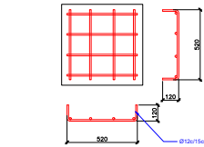
Detall riostra
