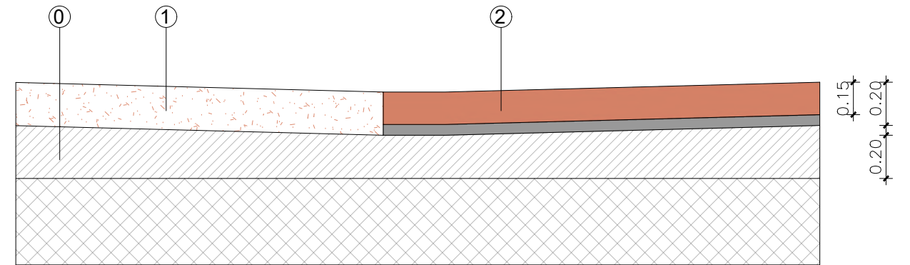
DETALL AA'
