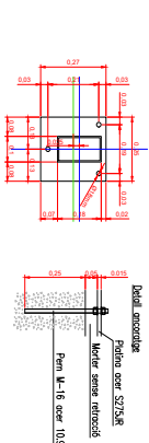
DETALL ABBONDONA TUBULAR 180x100x20mm (6 UNITS)
