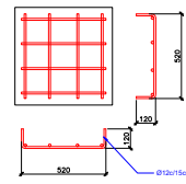
Detall riostra
