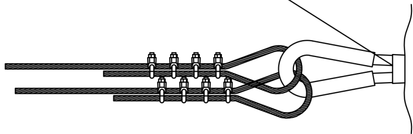
Detall 3 Extrems laterals
