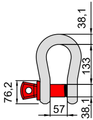
Grillete 3/8" SPIDER Y QUAROX
