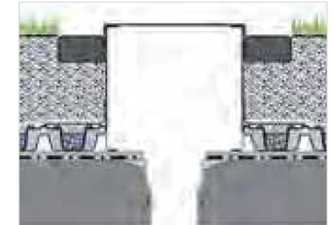
Caja de control KS 30/30-E
