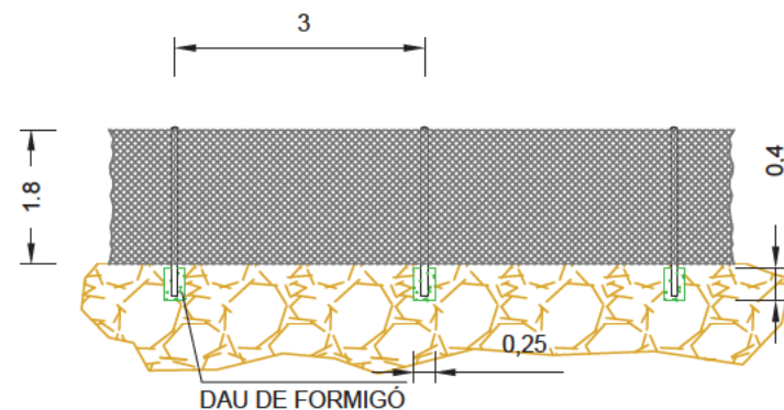
DETALL TANCA PERIMETRAL
