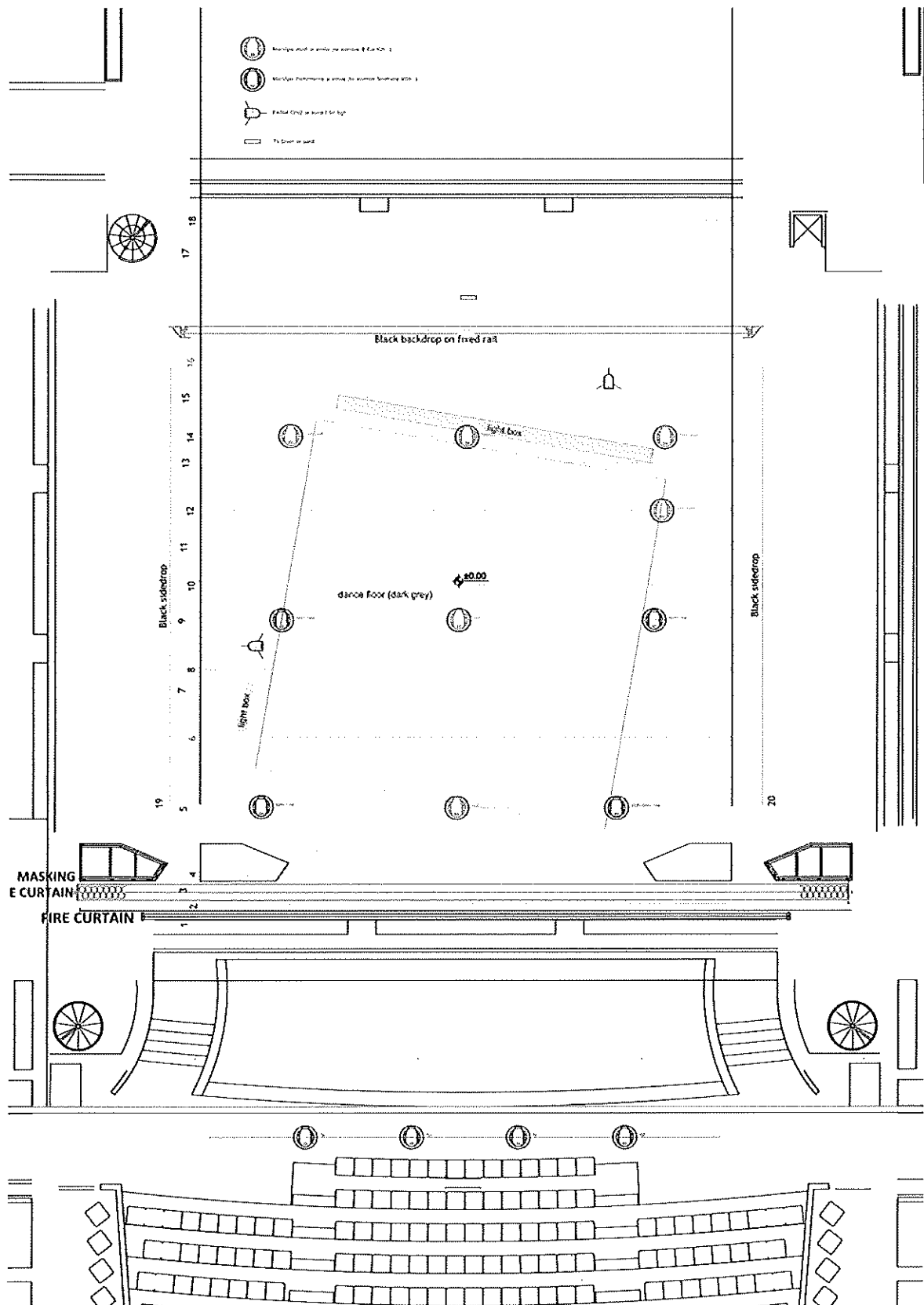
Set and light plot
