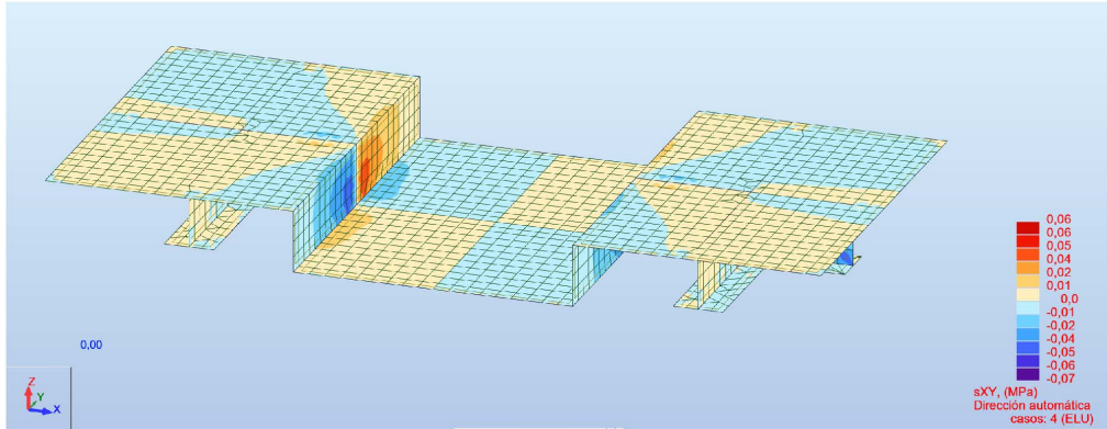
Sxy
