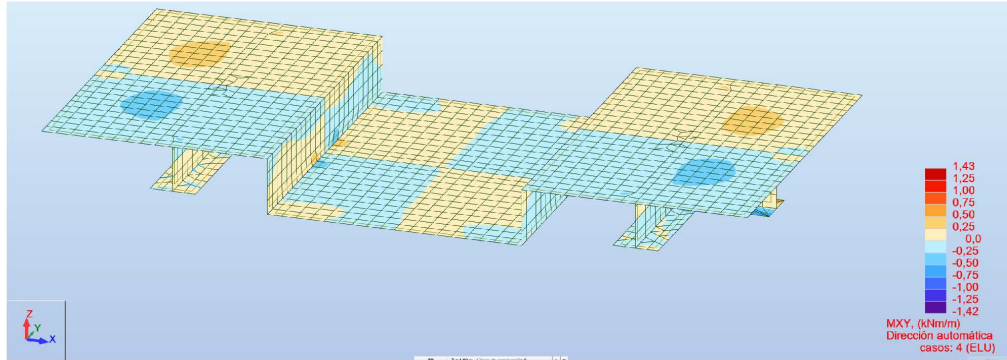
Mxy
