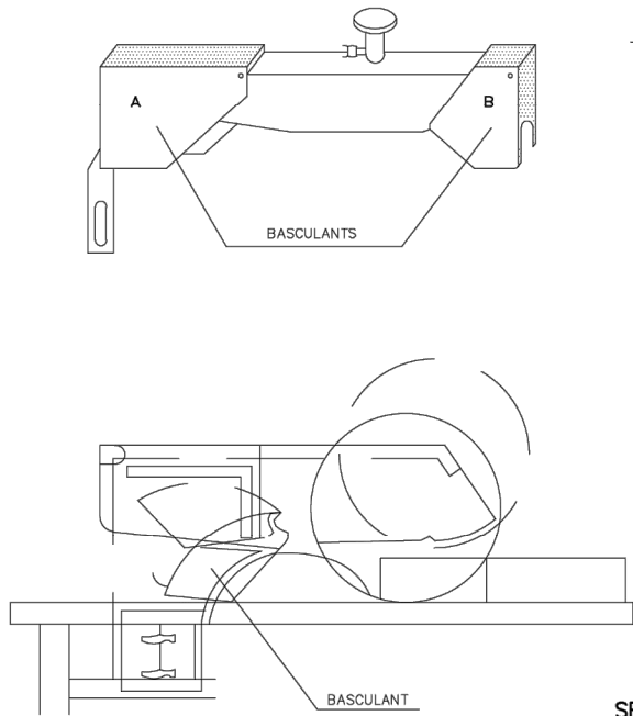
CARCASSES PROTECTORES
