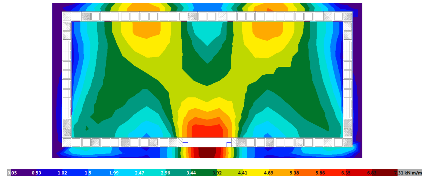
Figura 5. Moment X, quantia superior
