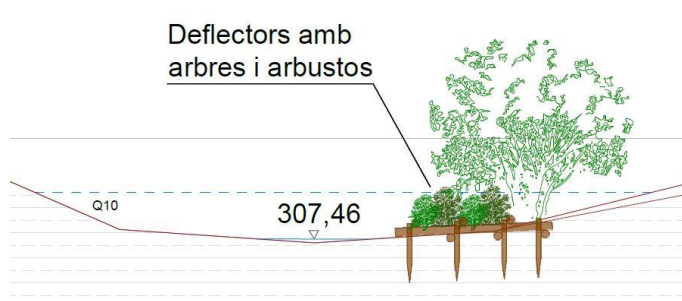
Figura 16 Deflectors vegetats
