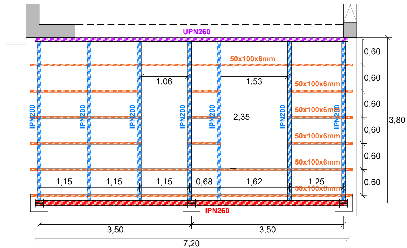
SOSTRE DE COBERTA - IPN260 + UPN260 / IPN200
