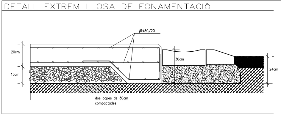
DETALL -2 e:1/20
