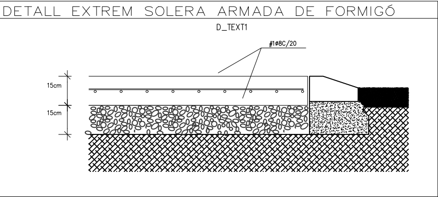
DETALL -1 e:1/20
