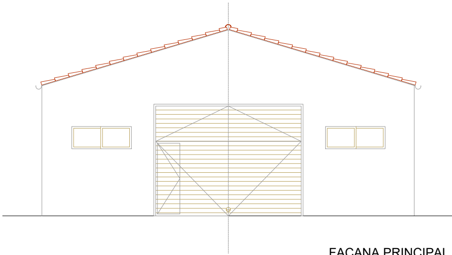
FAÇANA PRINCIPAL
