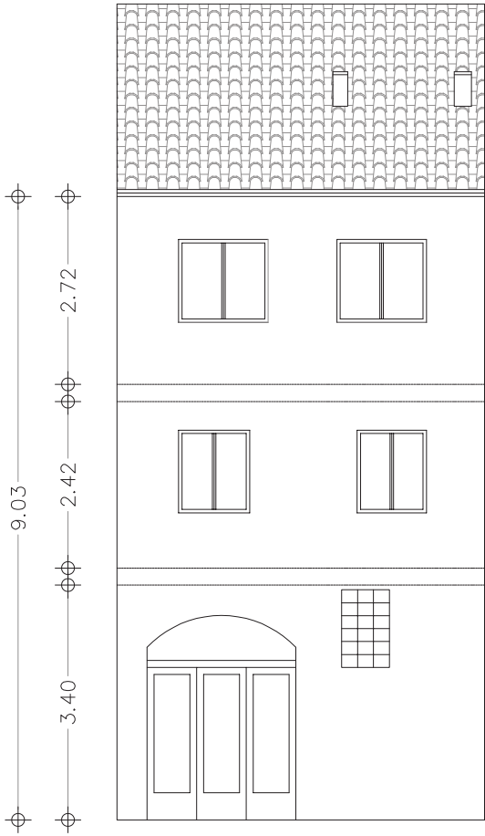
Façana Principal
