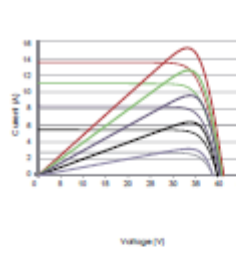
Current-Voltage & Power-Voltage Curves (450W)
