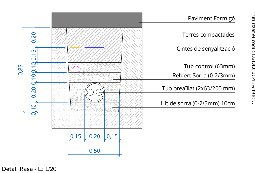
Detall Rasa - E: 1/20
