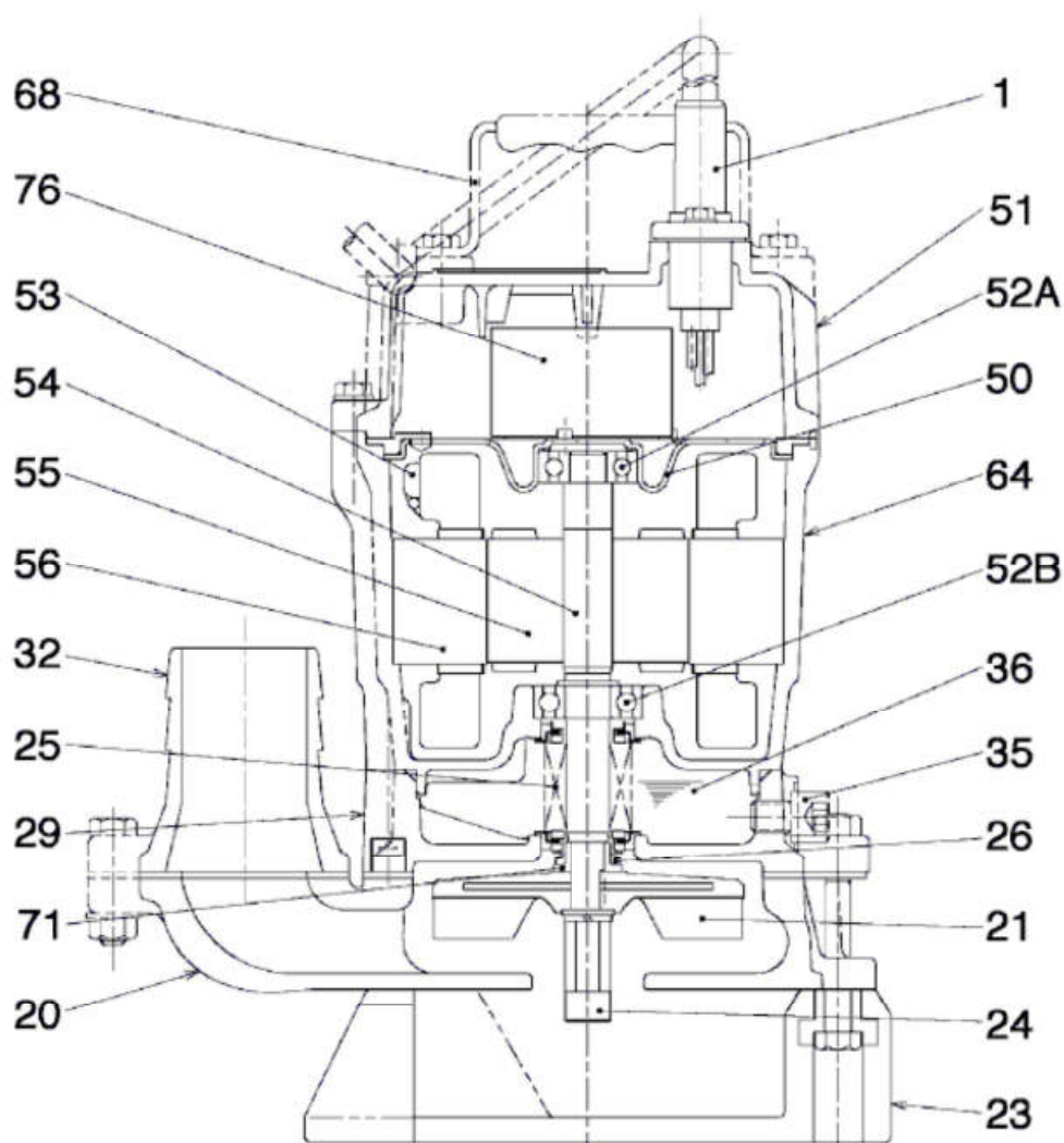
HS2.4S-52 (A-09153-1)
