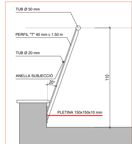
DETALL - Barana perimetral E: 1/20
