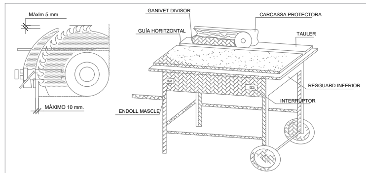
Carcasses protectores
