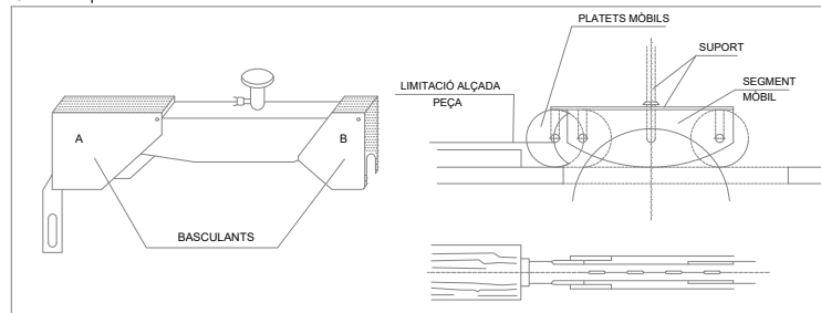
Serra circular
