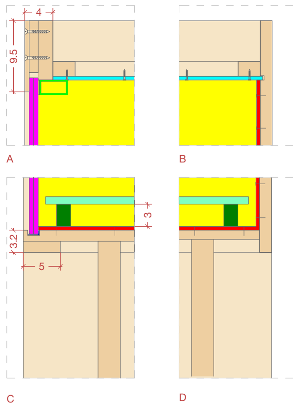
Detalls A,B,C i D - Escala 1:5 Interiors vitrines verticals
