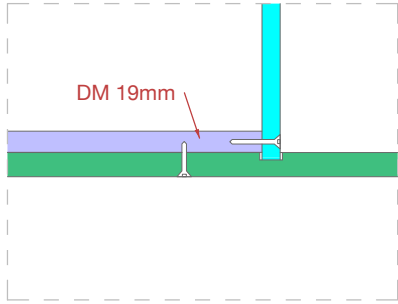
Detall B - Escala 1:5 Urna sense requeriments especials.
