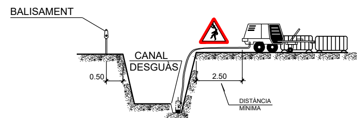
ESGOTAMENTS
