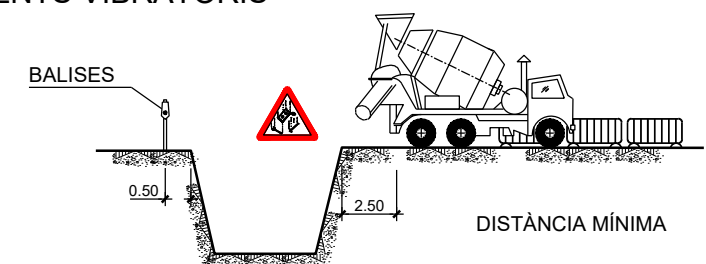
ELEMENTS VIBRATORIS
