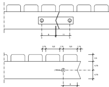
DETAILS E-10
