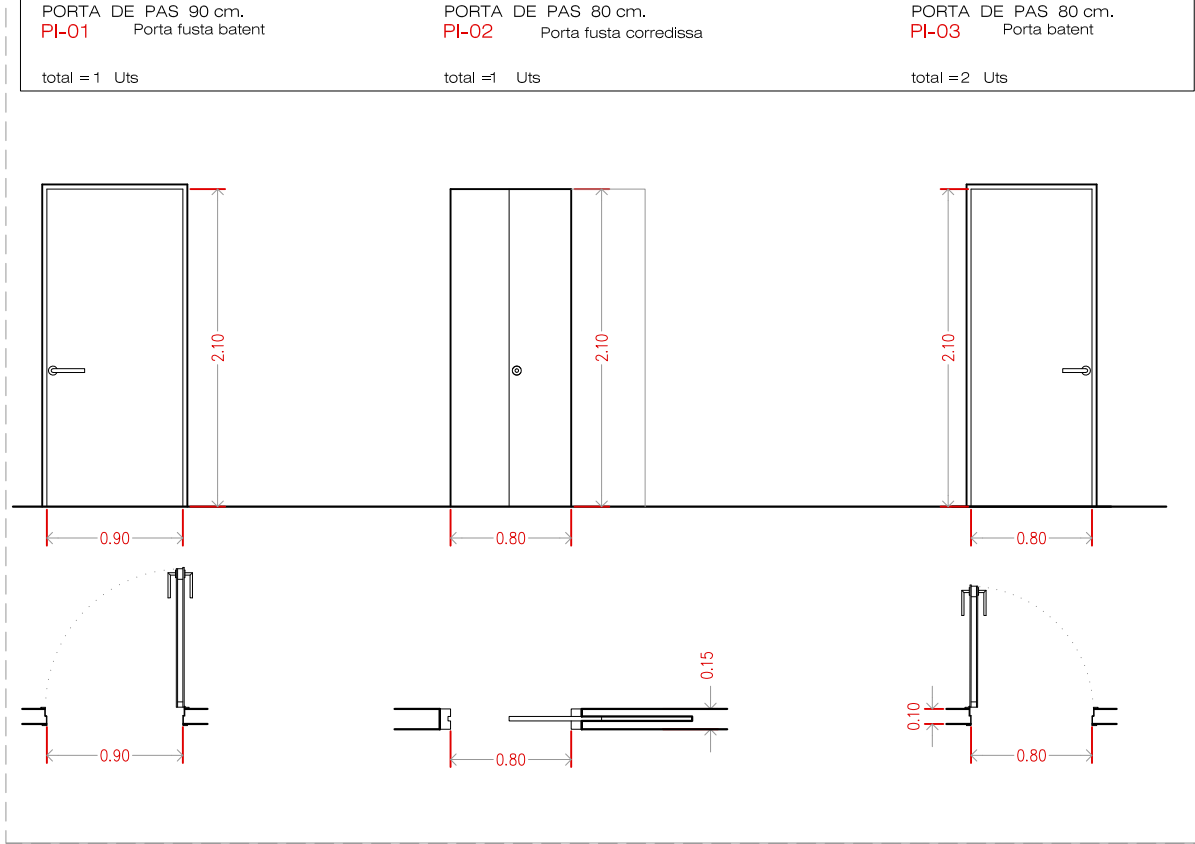
FUSTERIA INTERIOR
