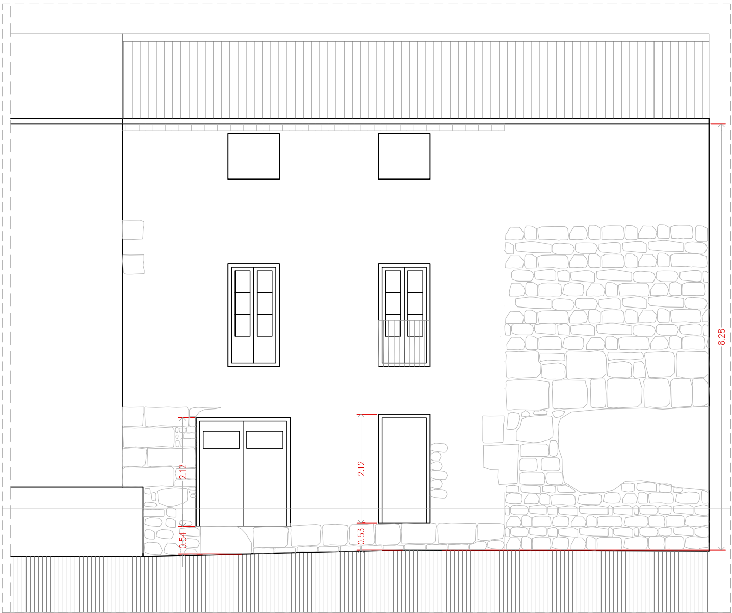
FAÇANA PRINCIPAL
