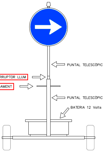
VISTA FRONTAL
