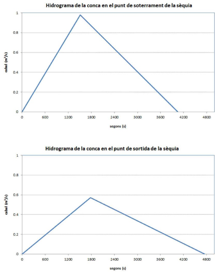
Figura 4. Hidrogrames resultants.
