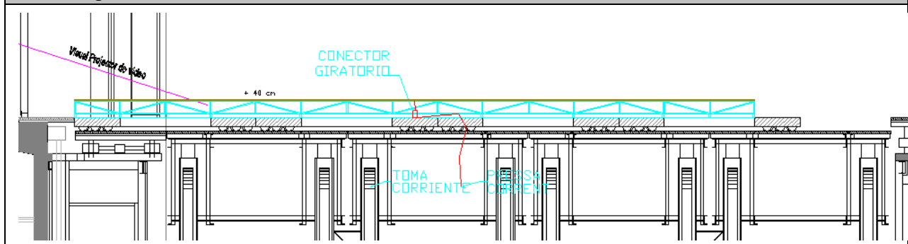
Revolving Platform Section Ø14,84m – Advanced Position 2m
