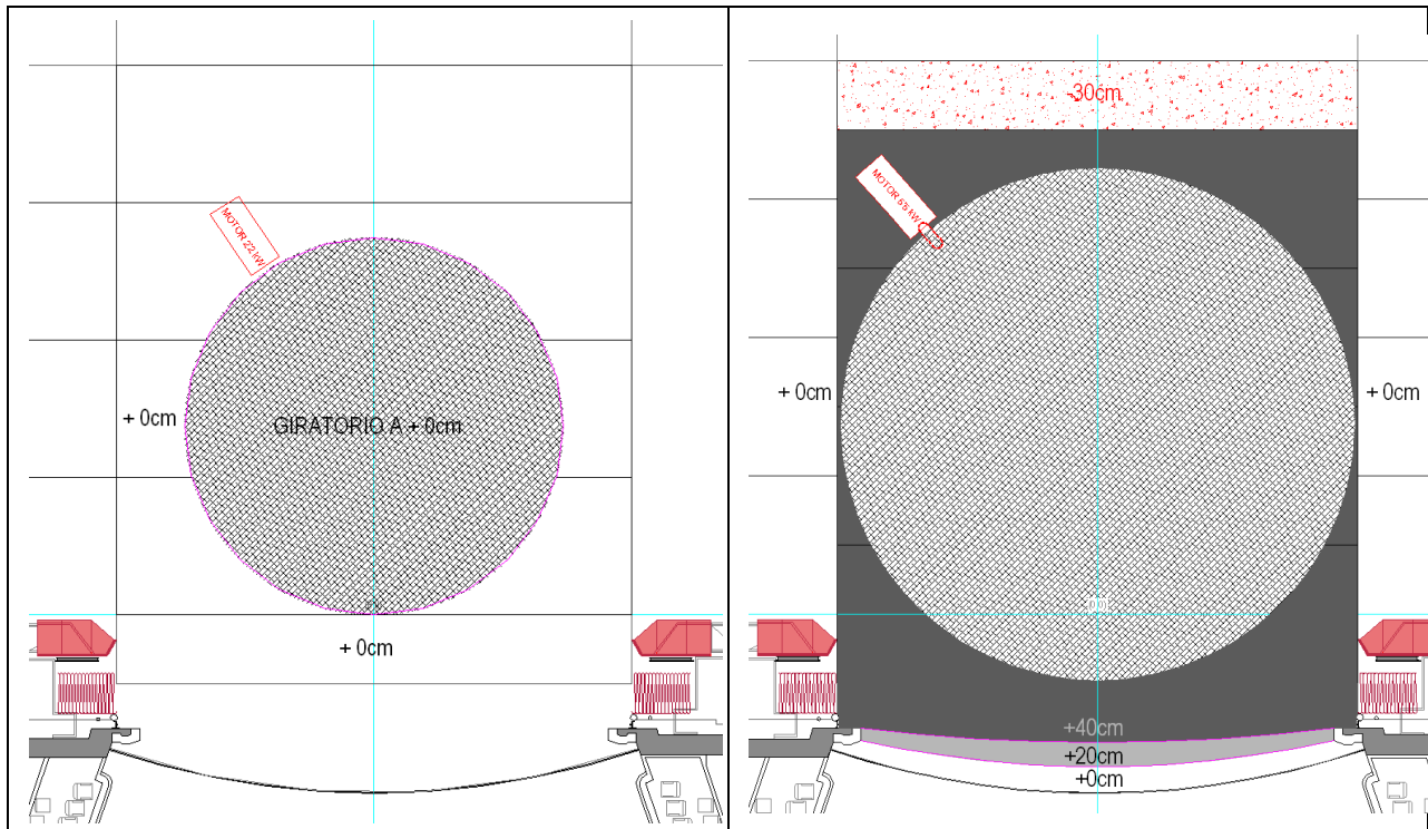
Revolving Platform Section Ø10,95m – Centred Position
