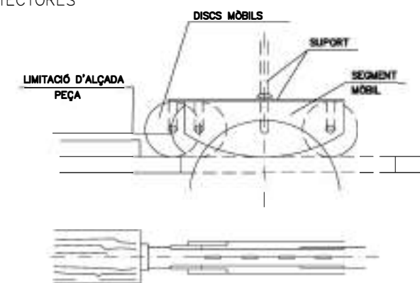
CARCASSES PROTECTORES
