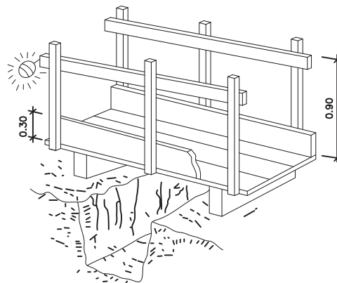
PASARELA PEATONAL
