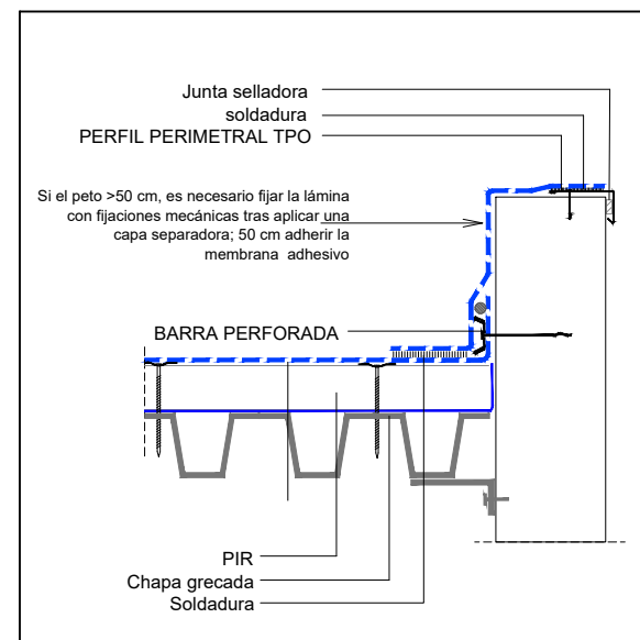
D4- DETALLE REMATE PERIMETRAL
