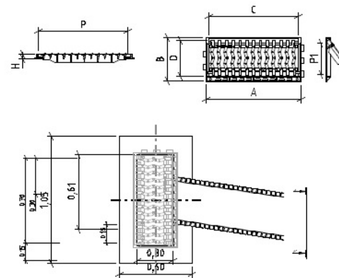
EMBORNAL MODEL ONA R0875
