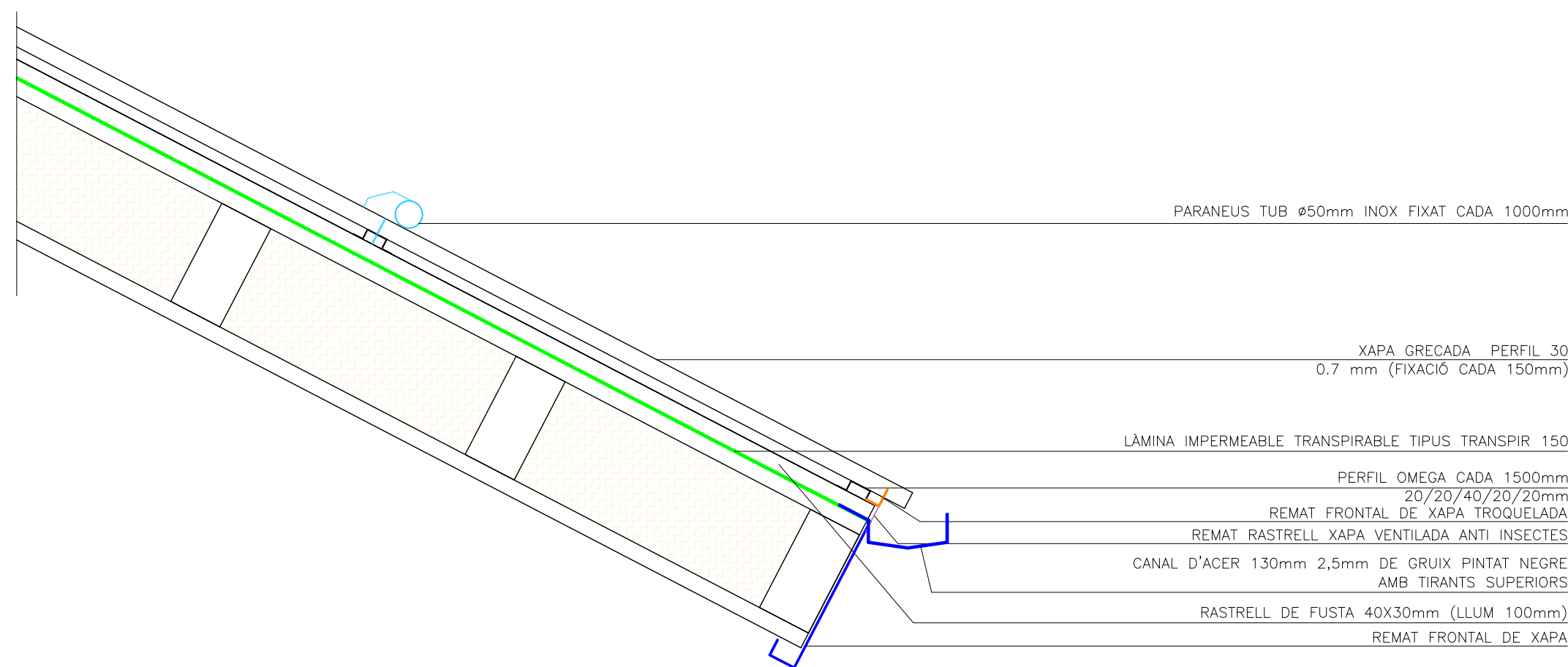
DETALL TUB PARANEUS Ø50mm
