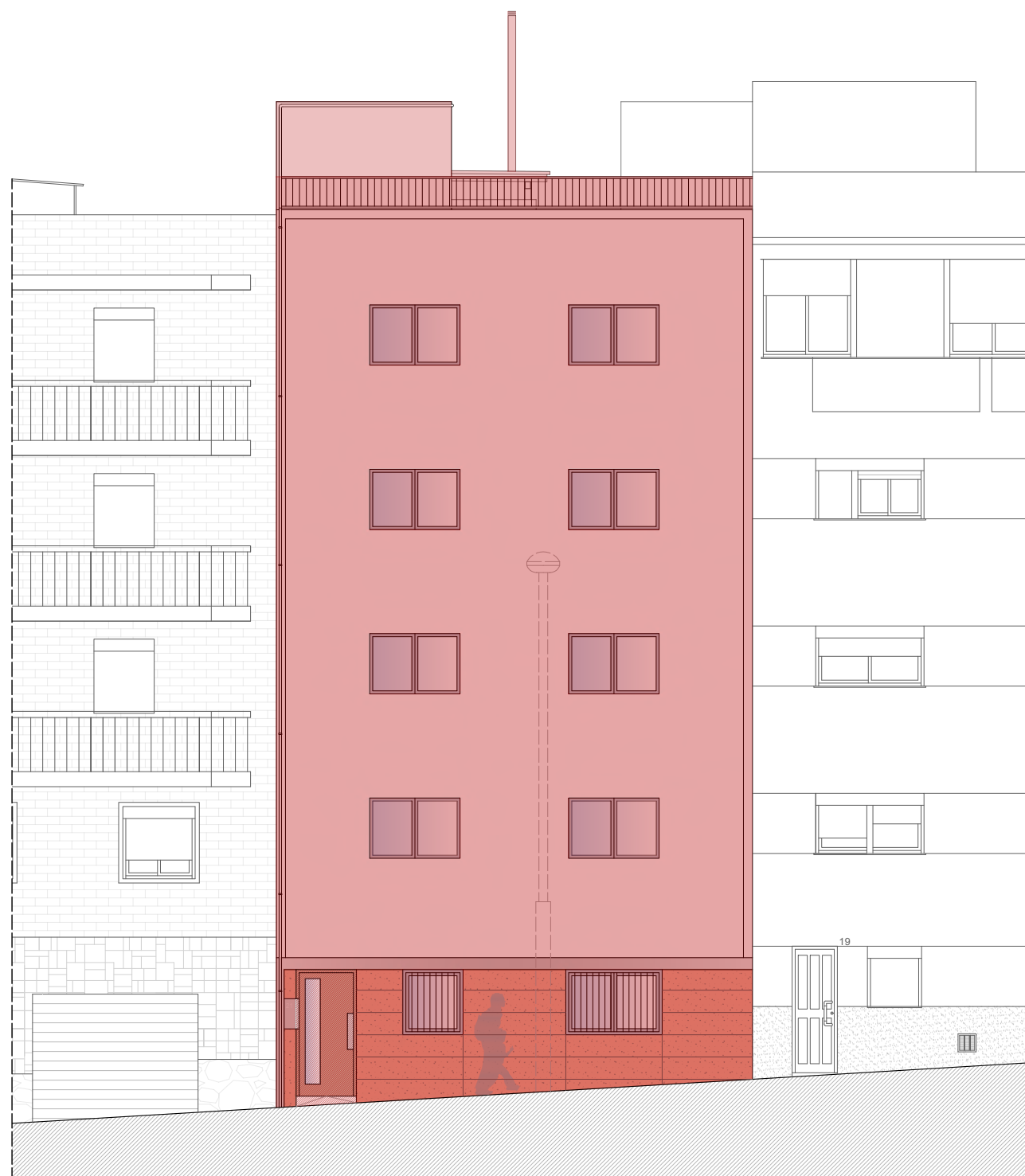
FAÇANA PRINCIPAL
